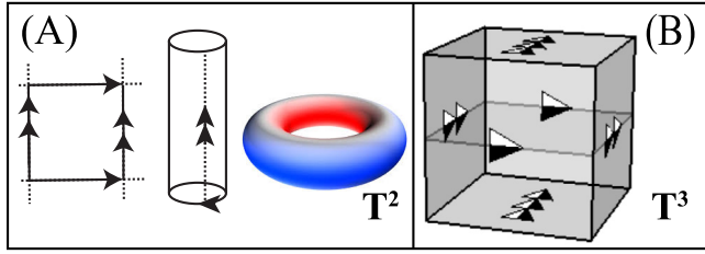
Figure 7. (A) A generic 2D Brillouin zone, with maximum wave-vectors k_x and k_y . Owing to periodic boundary conditions that apply to the first Brillouin zone, it has the topology of a two-dimensional torus T^2 . (B) A generic 3D Brillouin zone, with periodic boundary conditions.
