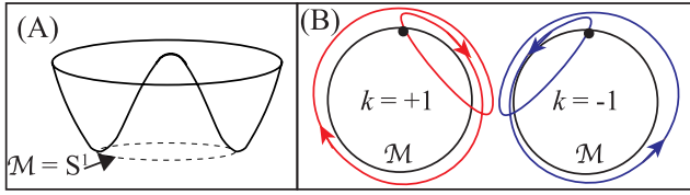
Figure 2. (A) The ‘Mexican hat’ potential energy configuration applies to complex ordered systems, below the bulk critical transition temperature. The manifold of degenerate ground states is the locus of points in the complex plane, i.e. \mathcal{M} = \mathbb{S}^1 . (B) \pi_1(\mathbb{S}^1) topological defects are available to complex ordered systems, by the specification of \theta on some closed loop. If, on taking a closed loop in space, \theta changes by 2\pi k ( k = 0, \pm 1, \pm 2, \dots is the winding number) then a defect core exists within the circuit.
