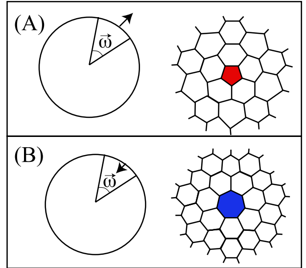
Figure 3. (A) Positive and (B) negative wedge disclinations in a honeycomb net. Wedge disclinations are characterized by a Frank vector ( \vec{w} ) topological invariant, on taking a measuring circuit around a point in space, and are the angular cousin to dislocations that are characterized by a linear Burger’s vector. An angular deficit attributes a topological strength to a wedge disclination, by introducing positive or negative curvature to it that is concentrated at its core.
