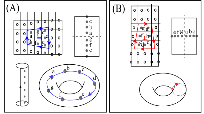
Figure 8. Dislocation fundamental homotopy group defects are permitted in crystalline solids. As a closed loop is traversed around a dislocation, the positions of atoms drift with respect to their ideal lattice positions. This corresponds to a loop around the order parameter space. Rearranging the atoms slightly deforms the loop, but does not change the number of times it wraps around the torus. (A) A loop around a dislocation that corresponds to an extra row of atoms corresponds to a path that passes around the hole of the torus. (B) A path through the hole of the torus corresponds to an extra column of atoms. Reproduced with permission of the Licensor through PLSclear, from [36]. Copyright Oxford University Press 2006.
