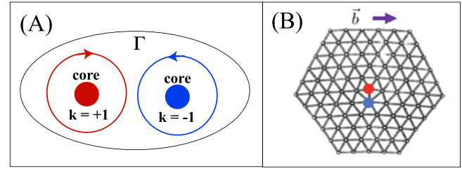
Figure 5. (A) A loop \Gamma that surrounds a pair of point defect cores whose topological invariants sum to zero is topologically equivalent to the uniform state, because \pi_m(S^m) defects are Abelian. (B) A dipole of positive and negative wedge disclinations, and the Burger's circuit and Burger's vector used to define the equivalent edge dislocation. (B) reprinted figure with permission from [15], copyright 2018 by the American Physical Society.
